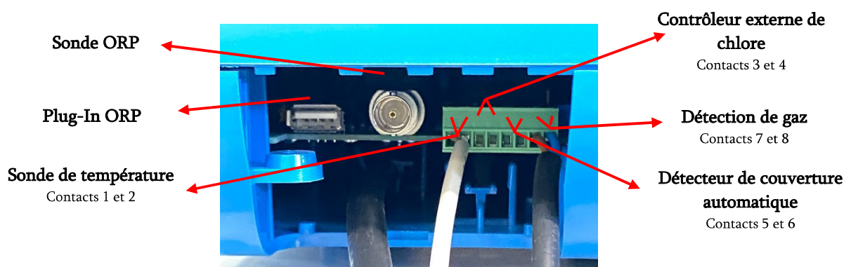
Figure 6 - Connexions internes
